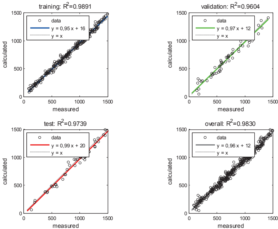
Figure 4: Results of a trained ANN [0,01 %] (example: Bremerhaven).
