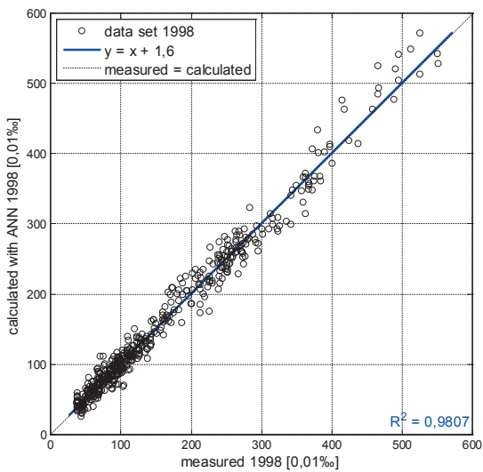
Figure 11: Scatter plot for calculated and measured salinities for gauge Strohauser Plate: data set from 1998 before waterway deepening.
