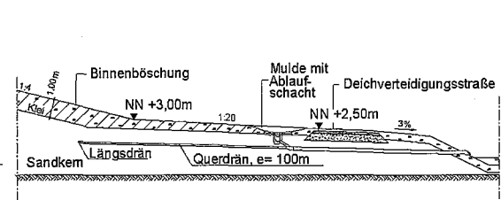
Detail Binnenberme
