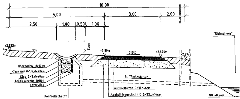
Detail C
