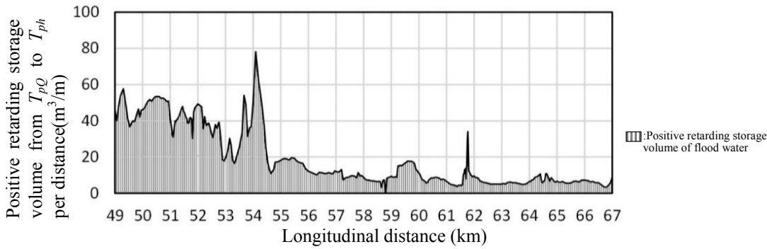
Figure 10. Longitudinal distribution of positive retarding storage volume from T_{pQ} to T_{ph} per unit distance.
