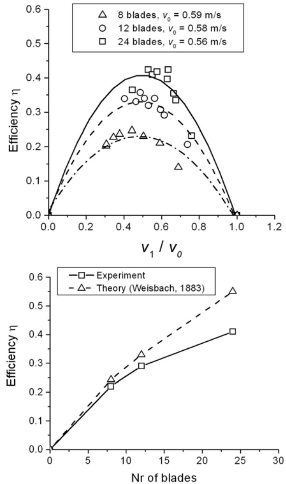
Fig. 6: Efficiency as function of blade number, Blockage reduction factor f_b = 1.3 , (a) Efficiency as function of velocity ratio v_1 / v_0 , (b) Experimental and theoretical efficiency
