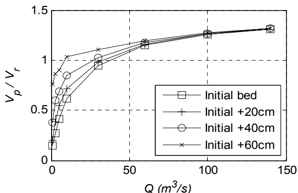
Figure 5. Velocity reversal index in PR2 as a function of flow discharge. Curves were obtained using the initial bed shape and increasing the elevation of the downstream riffle (at coordinate x=957m ) by 20, 40 and 60cm.
