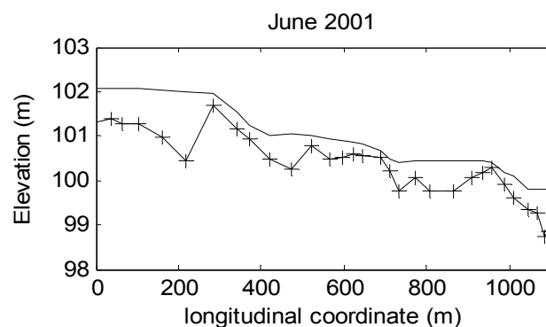
Figure 2. Initial bed and water surface profiles.
