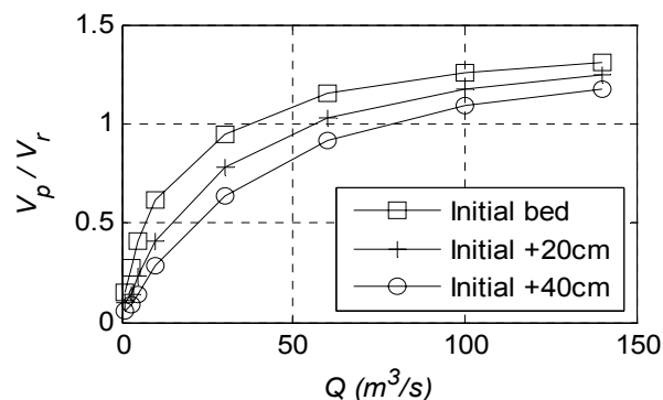
Figure 6. Velocity reversal index in PR2 as a function of flow discharge. Curves were obtained using the initial bed shape and increasing the elevation of the riffle at x=687m by 20 and 40cm.
