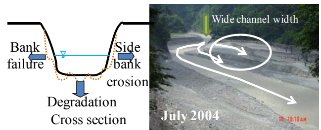
Figure 16. Flushing channel formed in Dashidaira reservoir
