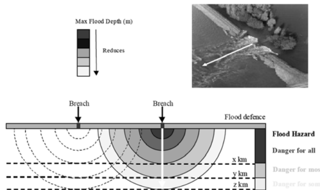
Figure 5. Flood areas due to breaching interpreted as danger to people (from Defra/EA 2005)
