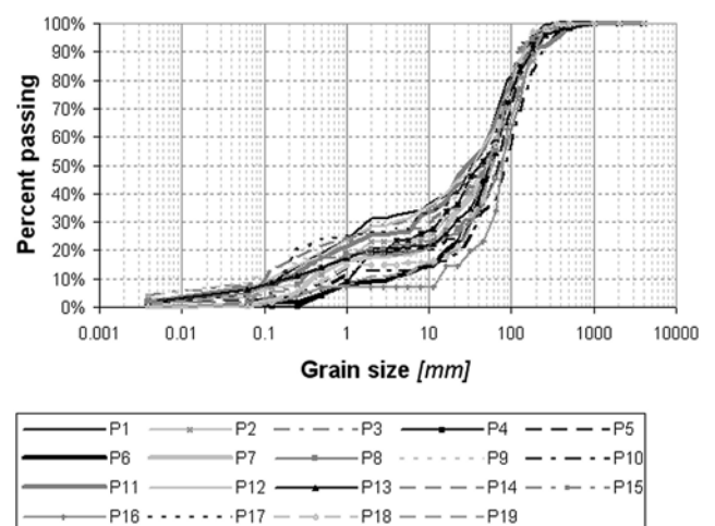
Figure 3. Grain size distribution curves at each transect
