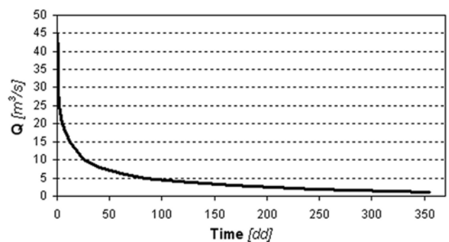
Figure 4. Study site flow duration curve.
