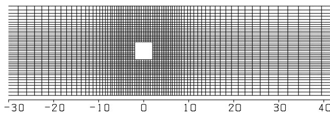
Figure 7. Computational grid used for 3D computation (Kimura et al. (2006)).
