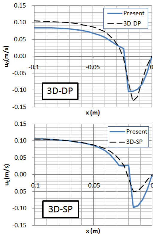
Figure 11. Predicted velocity profiles at the bed around a square cylinder by the present model (upper: 3D-DP, lower: 3D-SP).
