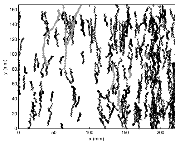
Figure 5. Sample trajectories used for the trajectory-based validation of the PTV measurements (top). Sub-sample of the obtained trajectories (only those with duration larger than 0.2 s) with the blob (middle) and grey images (bottom).
