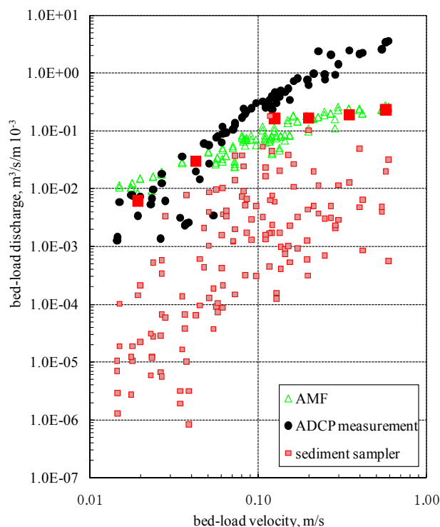
Figure 4 Relationship between the bed-load velocity and bed-load discharge (several dots of the sediment sampler highlighted as larger dots)
