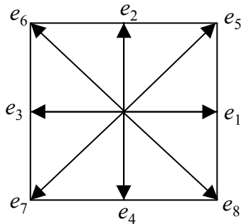
Bild 10.2 The eight unit vectors \mathbf{e}_i pointing to the nearest neighbouring site in direction i .
