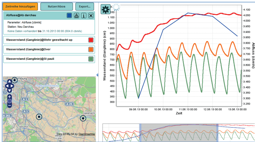
Figure 5: Sensor Web Client time series display – extreme flood event in Geesthacht on the River Elbe – water level and discharge parameters.
