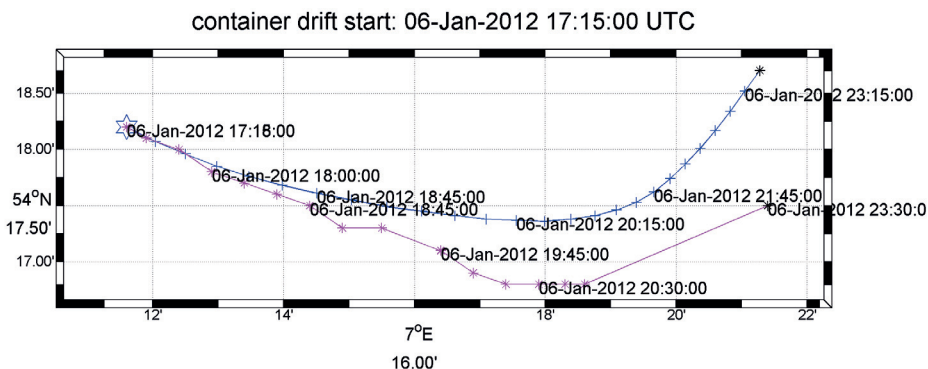
Figure 5: Seatrack web drift trajectory (blue) and observed trajectory (magenta) of two connected containers starting from a ship observed position ( 54^{\circ} 18,2'N , 007^{\circ} 11,6'E ) at 06.01.2012 at 17:15 UTC ending at 06.01.2012 at 23:30 UTC (plot is made with Matlab). The star marks the starting point of the simulation. Seatrack Web uses a wind drag coefficient of 2.3 %.
