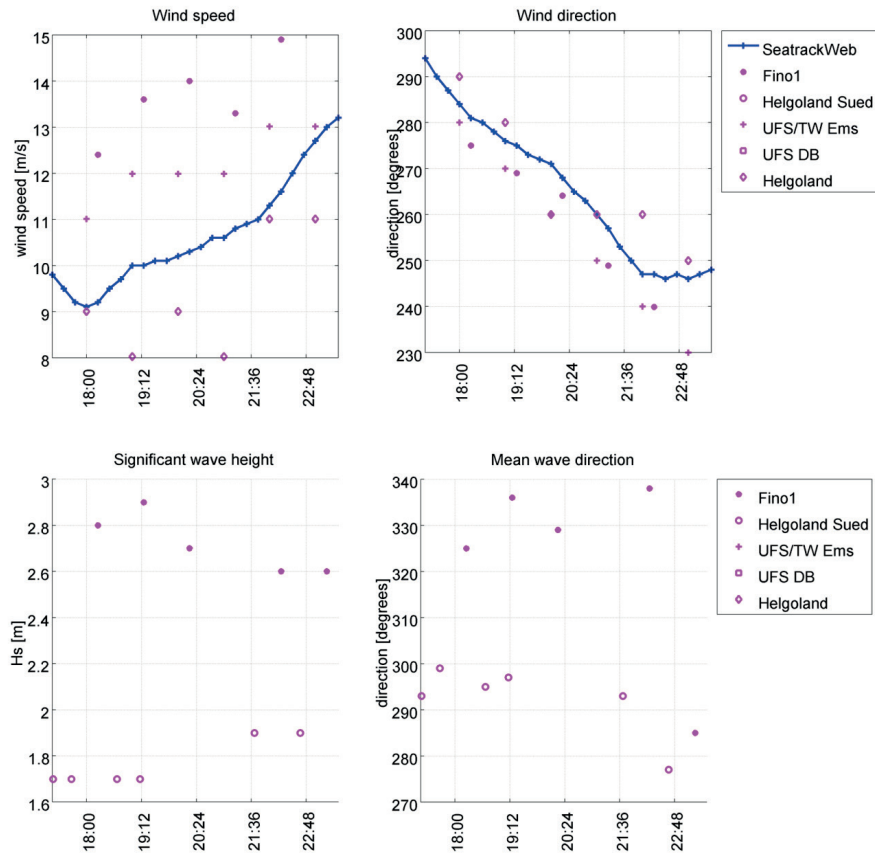
Figure 6: In blue wind speed and wind direction (in 10 m height) over time used by the drift model (GME+LME model data) at the simulated container positions. The dots in magenta show wind speed, wind direction, significant wave height and mean wave direction as measured at the station Fino1 ( 54^{\circ} 0.86' \text{ N} , 006^{\circ} 35.03' \text{ E} ). The wind measurements of Fino1 are in 33 m height. The magenta circles show significant wave height and mean wave direction from the wave buoy at Helgoland Sued ( 54^{\circ} 10.783' \text{ N} , 007^{\circ} 53.467' \text{ E} ). Wind speed and direction measurements at light vessel TW Ems ( 54^{\circ} 10.0' \text{ N} , 006^{\circ} 20.8' \text{ E} ) in magenta crosses and at Helgoland in magenta diamonds.
