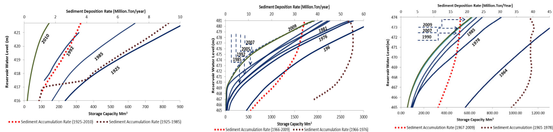
Figure 4: Reservoirs sedimentation and sediment accumulation rate for (a) Sennar, (b) Roseires, and (c) Girba dams.
