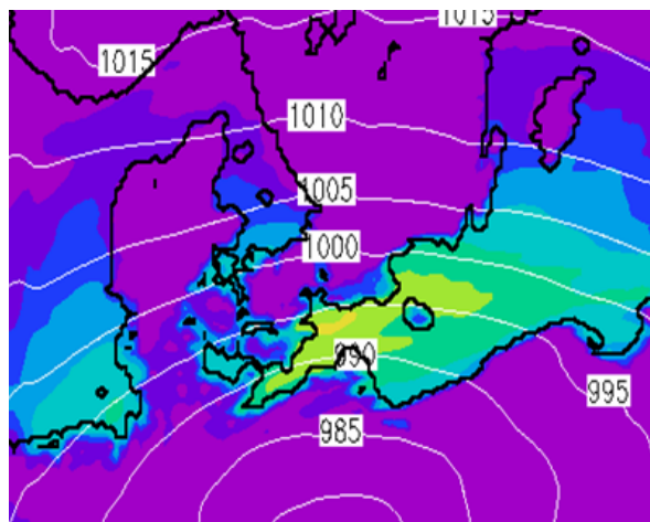
d) EPS Nr.45, +179h
