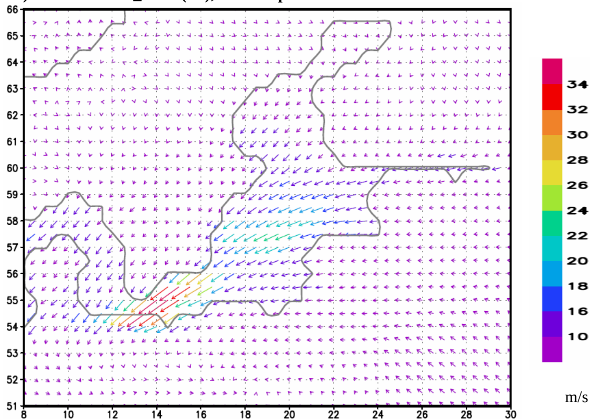
a) Member Nr.35_b0cw (sfc); Startzeitpunkt 11.11.1970 12 UTC + 164h
