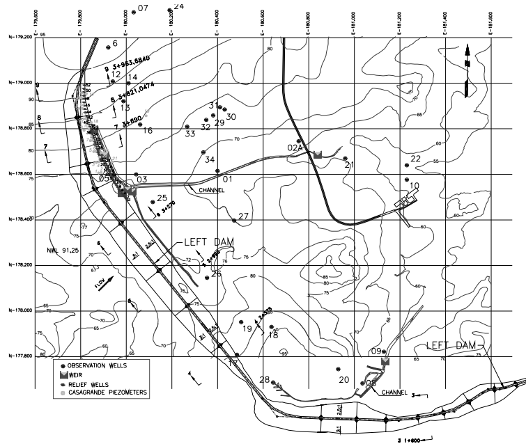
Figure 4. Map showing locations of piezometric head sensing devices and weirs for flow measurements.
