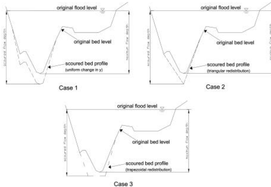
Figure 1. Scoured channel profiles used in Test cases 1, 2 and 3.
