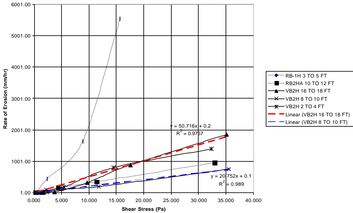
Figure 7. EFA Test Results plotted on a natural scale.
