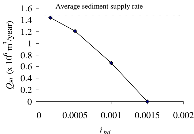
Fig.3 Relation between the allowable sand mining volume, Q_{sa} , and the designed bed slope, i_{bd}
