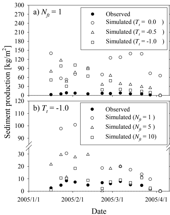
Fig. 10 Simulated sediment production: a) Necessary number of freeze and thaw cycle, N_{ft} , was fixed to be 1, b) Threshold temperature for freezing, T_i , was fixed to be -1.0 degree C
