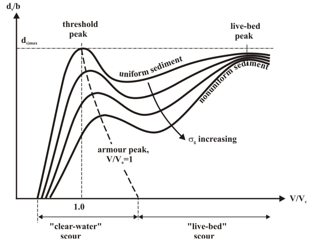
Fig.1 Local scour depth variation with flow intensity
