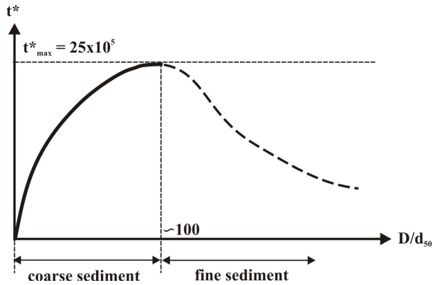
Fig.7 Equilibrium time scale variation with flow shallowness, flow intensity and sediment coarseness
